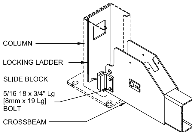
Fig 9 – Slide Block Installation
