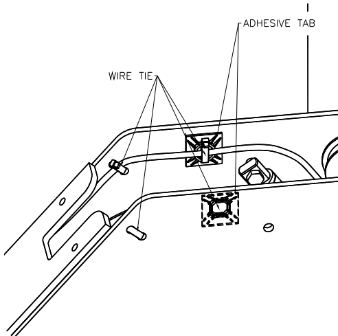
Fig 13 – 4mm Air Line Connection
