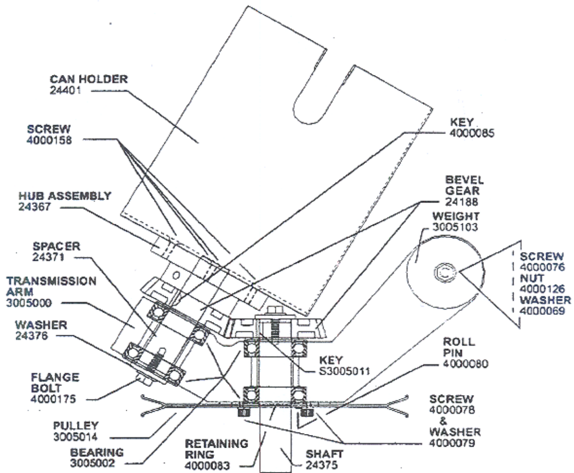
Figure 5 Transmission Arm Assembly
