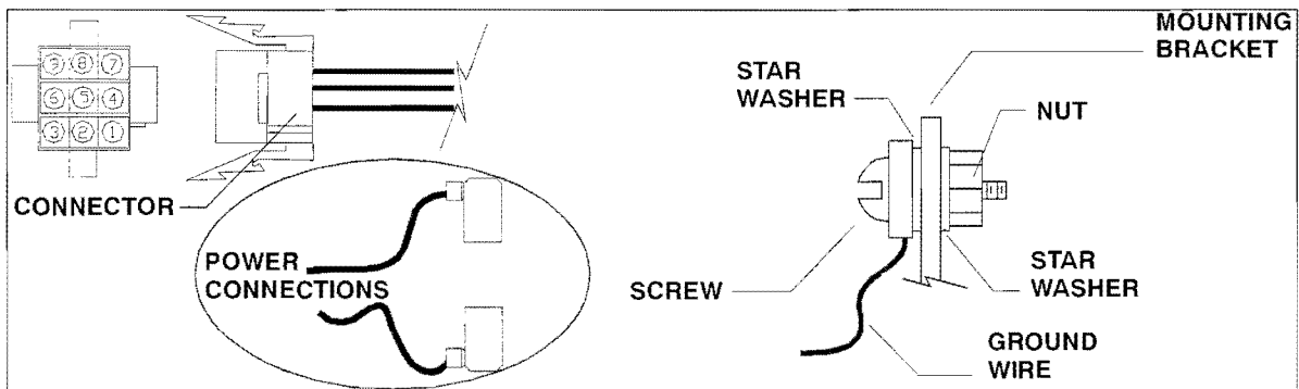
Figure 3 GQB Wiring
