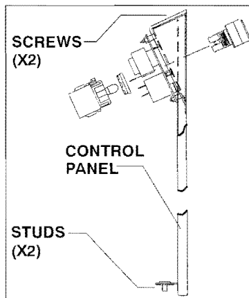
Figure 4 GQB Panel
